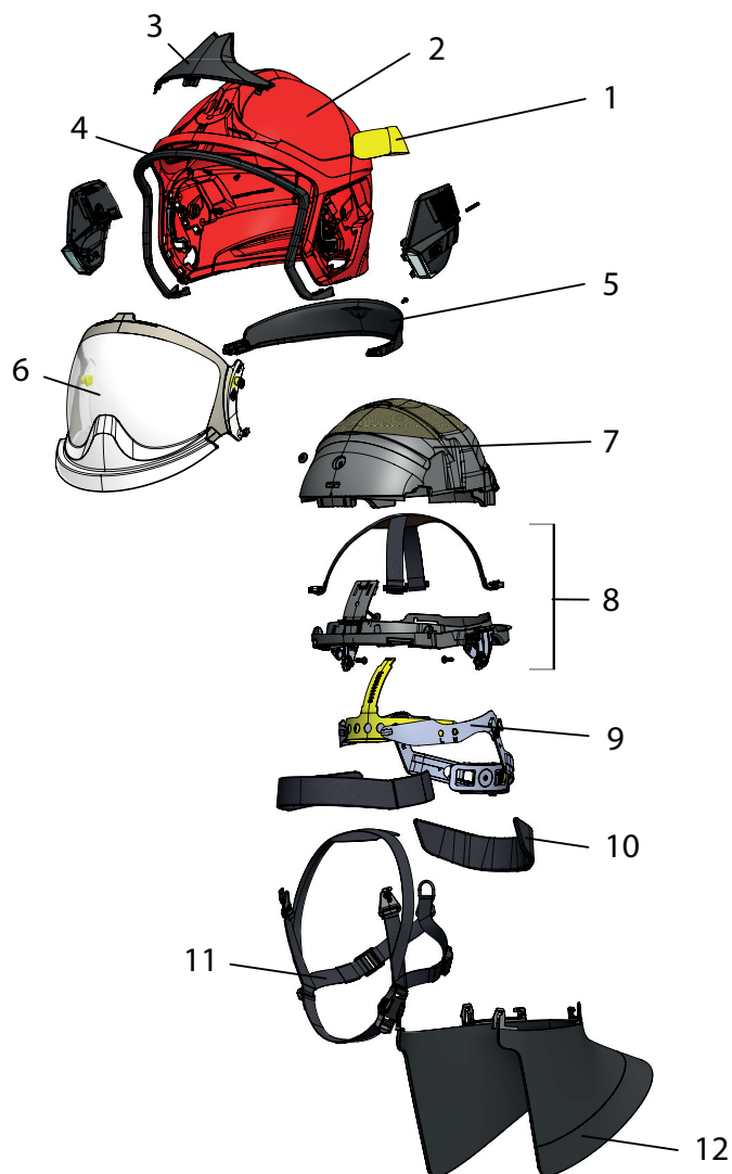
Fig. 1 Exploded view
