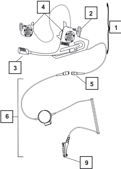
Figure 1 Micro-casque flexible
