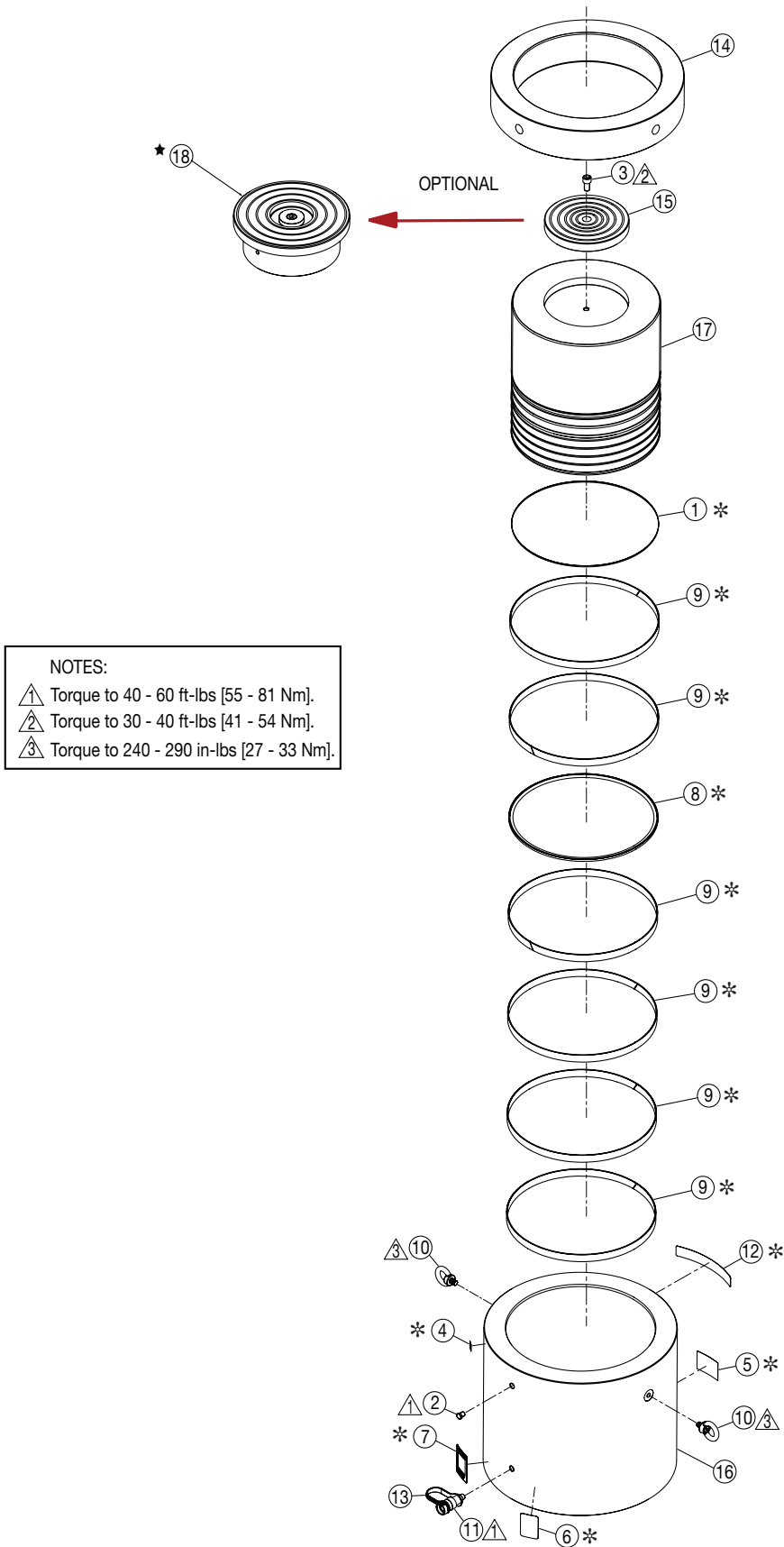
Figure 3, Exploded View - Model HCL-1000
