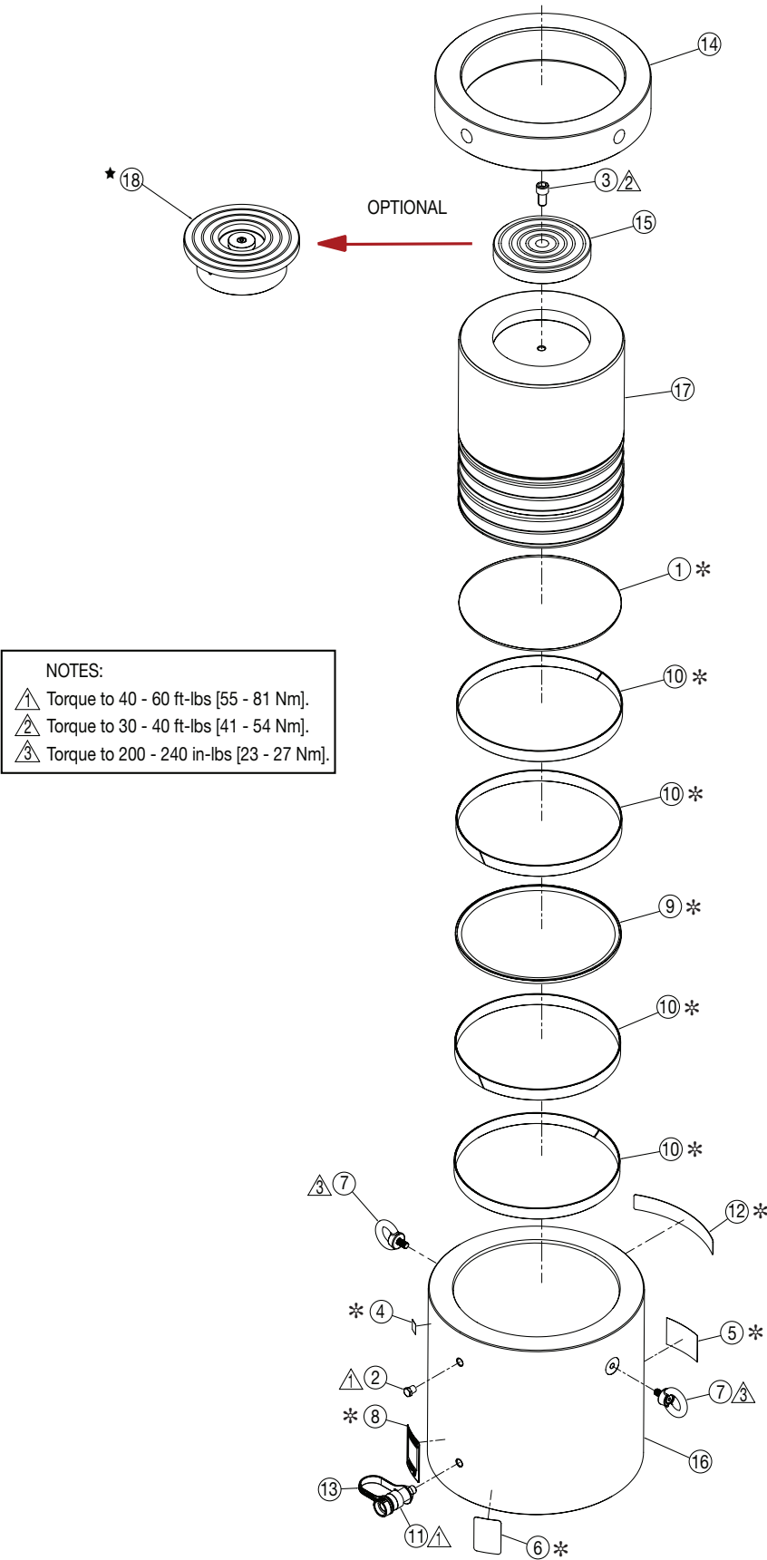
Figure 1, Exploded View - Model HCL-600
