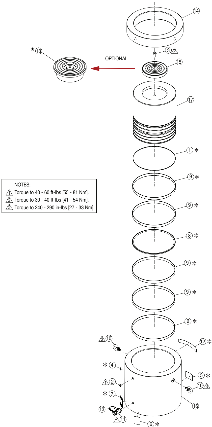
Figure 2, Exploded View - Model HCL-800
